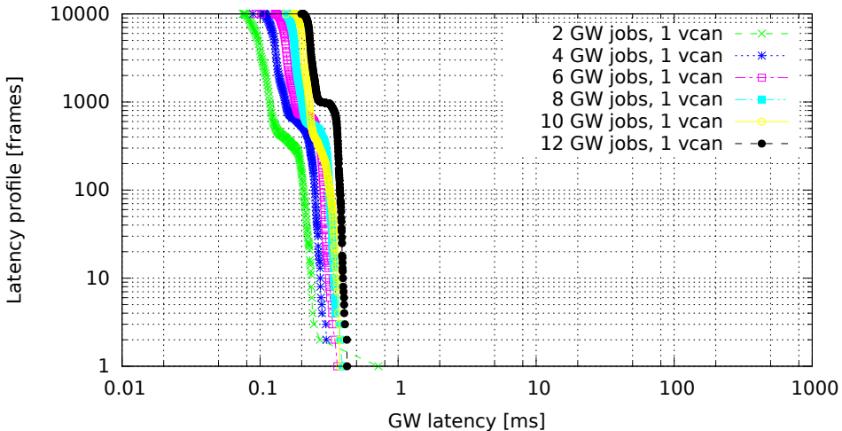
Chained GWs on a single VCAN interface (GW kernel 2.6.36.2-00015-g4f1bc4e, Traffic oneatatime, Load cpu)
