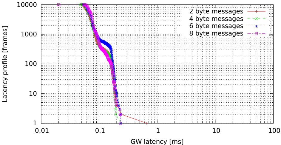
Single GW rule for all messages, no modifications, high (soft)irq task priority (GW kernel 2.6.36.2-00015-g4f1bc4e, Traffic oneatatime, Load cpu)
