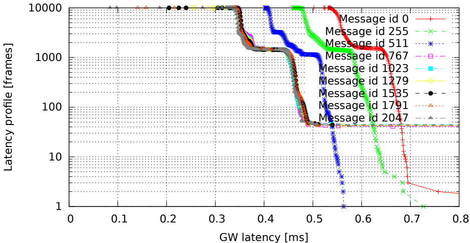
2048 GW rules (one per id, mask 0x7FF), no modifications (GW kernel 2.6.36.2-00015-g4f1bc4e, Traffic oneatatime, Load cpu)
