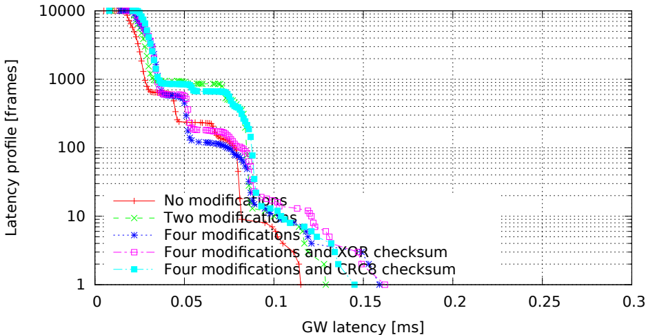
Single GW rule for all messages with modifications, 8 byte messages (GW kernel 2.6.36.2-00015-g4f1bc4e, Traffic flood, Load none)
