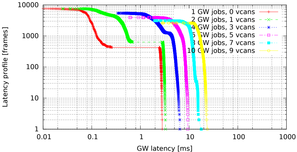
Chained GWs on multiple VCAN interfaces (GW kernel 2.6.36.2-00015-g4f1bc4e, Traffic flood, Load eth)
