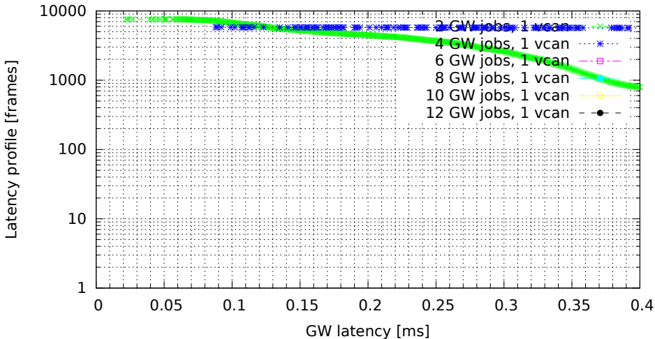
Chained GWs on a single VCAN interface (GW kernel 2.6.36.2-00015-g4f1bc4e, Traffic flood, Load eth)
