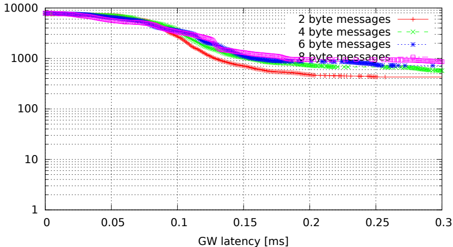
Single GW rule for all messages, no modifications (GW kernel 2.6.36.2-00015-g4f1bc4e, Traffic flood, Load eth)
