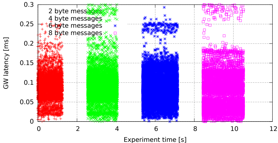
Single GW rule for all messages, no modifications (GW kernel 2.6.36.2-00015-g4f1bc4e, Traffic flood, Load eth)
