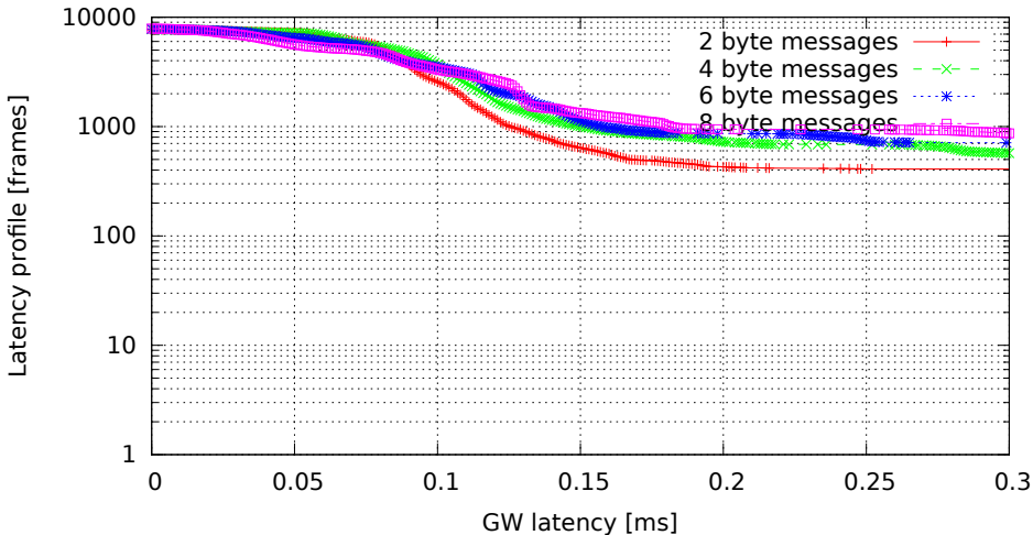
Single GW rule for all messages, no modifications, high (soft)irq task priority (GW kernel 2.6.36.2-00015-g4f1bc4e, Traffic flood, Load eth)
