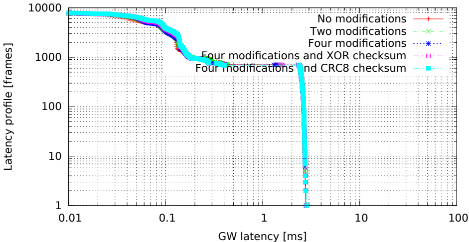
Single GW rule for all messages with modifications, 8 byte messages (GW kernel 2.6.36.2-00015-g4f1bc4e, Traffic flood, Load eth)
