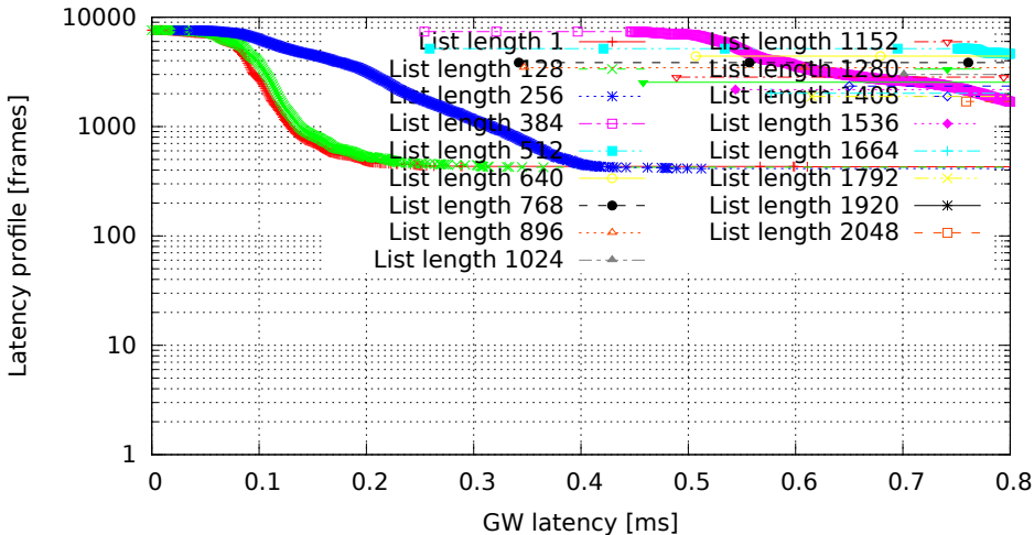
Different lengths of filter list, only the last one matches (GW kernel 2.6.36.2-00015-g4f1bc4e, Traffic flood, Load eth)
