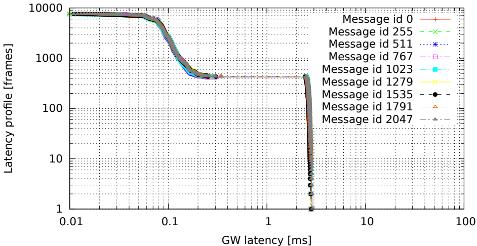
2048 GW rules (one per id, mask C00007FF), no modifications (GW kernel 2.6.36.2-00015-g4f1bc4e, Traffic flood, Load eth)
