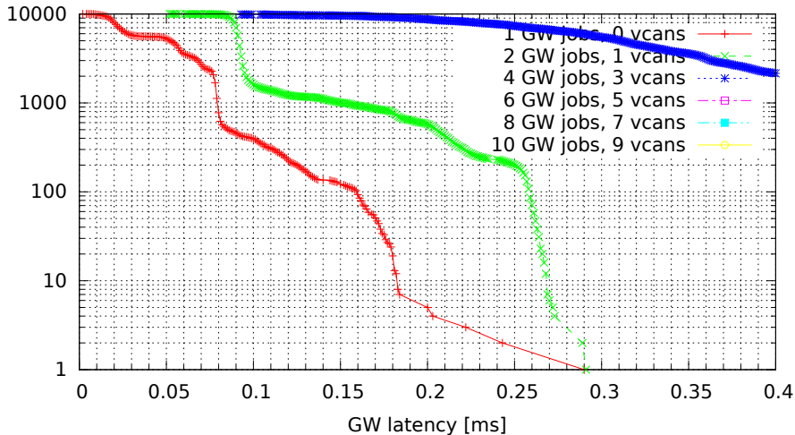
Chained GWs on multiple VCAN interfaces (GW kernel 2.6.36.2-00015-g4f1bc4e, Traffic flood, Load cpu)
