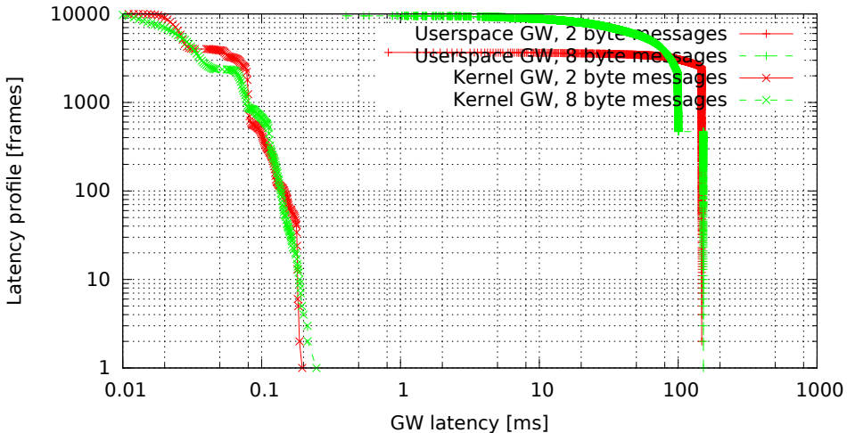
Kernel vs. userspace GW, no modifications (GW kernel 2.6.36.2-00015-g4f1bc4e, Traffic flood, Load cpu)
