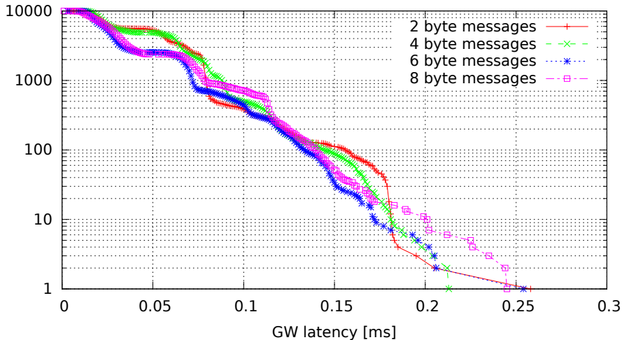
Single GW rule for all messages, no modifications (GW kernel 2.6.36.2-00015-g4f1bc4e, Traffic flood, Load cpu)
