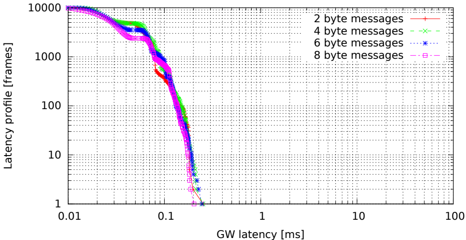
Single GW rule for all messages, no modifications, high (soft)irq task priority (GW kernel 2.6.36.2-00015-g4f1bc4e, Traffic flood, Load cpu)
