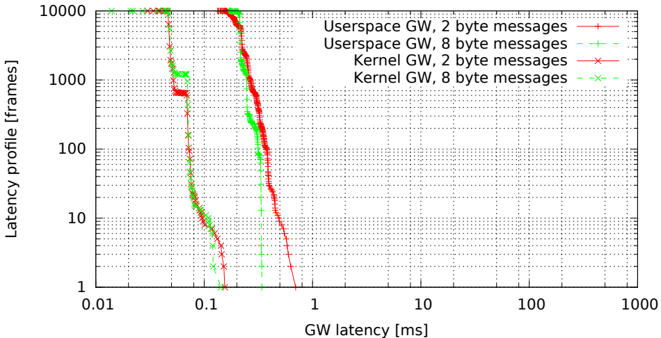
Kernel vs. userspace GW, no modifications (GW kernel 2.6.36.2-00015-g4f1bc4e, Traffic 50, Load none)
