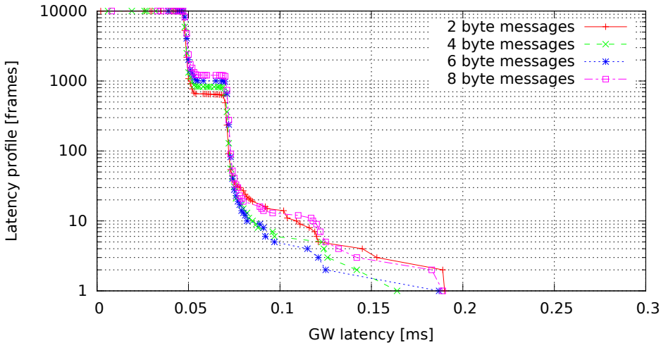
Single GW rule for all messages, no modifications, high (soft)irq task priority (GW kernel 2.6.36.2-00015-g4f1bc4e, Traffic 50, Load none)
