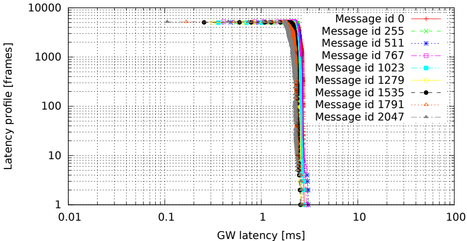
2048 GW rules (one per id, mask 0x7FF), no modifications (GW kernel 2.6.36.2-00015-g4f1bc4e, Traffic 50, Load none)
