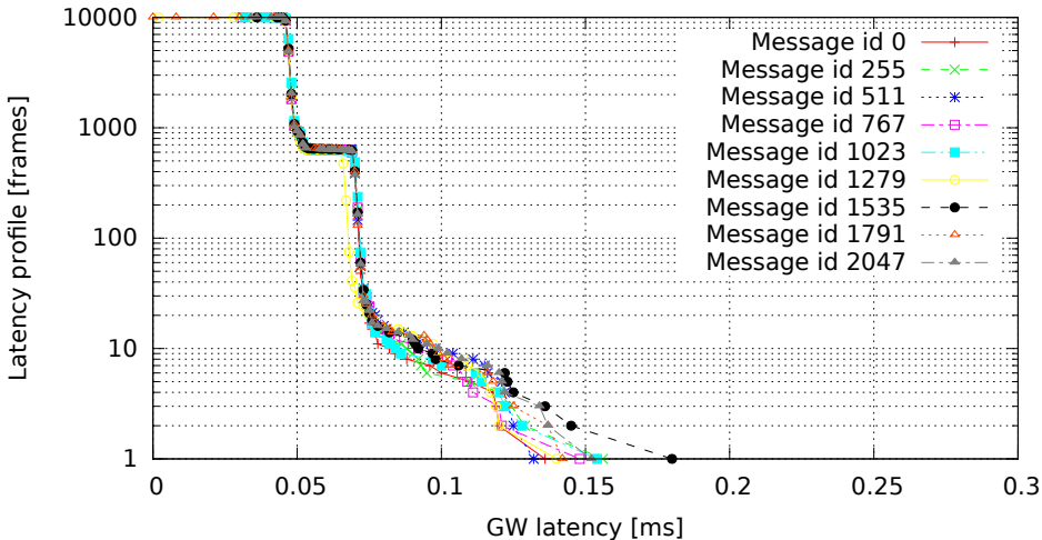
2048 GW rules (one per id, mask C00007FF), no modifications (GW kernel 2.6.36.2-00015-g4f1bc4e, Traffic 50, Load none)
