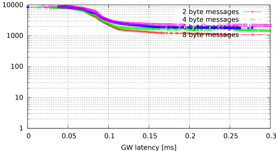
Single GW rule for all messages, no modifications, high (soft)irq task priority (GW kernel 2.6.36.2-00015-g4f1bc4e, Traffic 50, Load eth)
