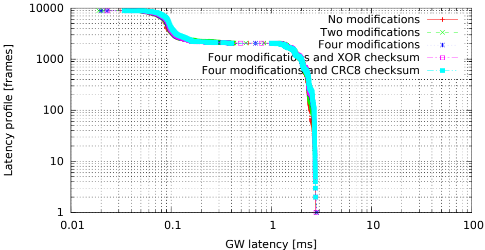
Single GW rule for all messages with modifications, 8 byte messages (GW kernel 2.6.36.2-00015-g4f1bc4e, Traffic 50, Load eth)
