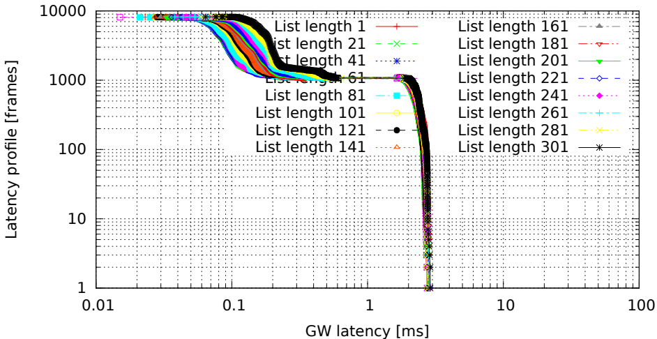
Different lengths of filter list, only the last one matches (GW kernel 2.6.36.2-00015-g4f1bc4e, Traffic 50, Load eth)
