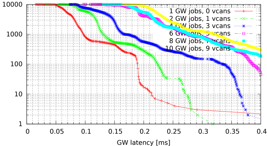
Chained GWs on multiple VCAN interfaces (GW kernel 2.6.36.2-00015-g4f1bc4e, Traffic 50, Load cpu)
