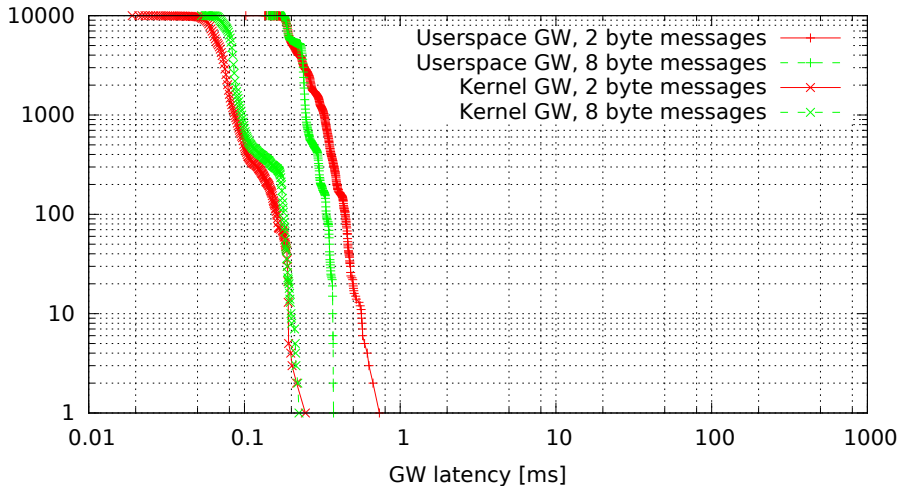
Kernel vs. userspace GW, no modifications (GW kernel 2.6.36.2-00015-g4f1bc4e, Traffic 50, Load cpu)
