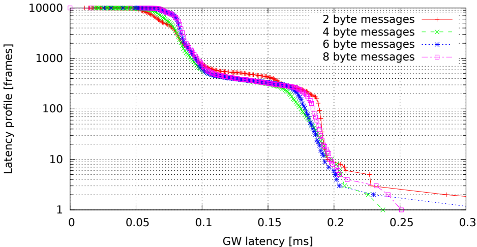
Single GW rule for all messages, no modifications, high (soft)irq task priority (GW kernel 2.6.36.2-00015-g4f1bc4e, Traffic 50, Load cpu)
