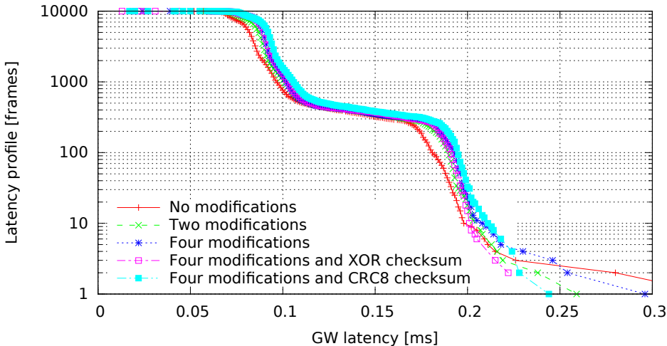
Single GW rule for all messages with modifications, 8 byte messages (GW kernel 2.6.36.2-00015-g4f1bc4e, Traffic 50, Load cpu)
