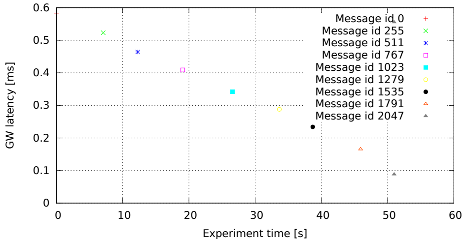
2048 GW rules (one per id, mask 0x7FF), no modifications (GW kernel 2.6.36.2-00015-g4f1bc4e, Traffic 50, Load cpu)
