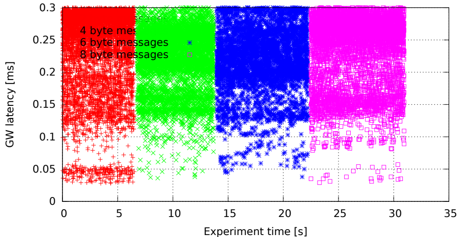
Single GW rule for all messages, no modifications (GW kernel 2.6.33.7-rt29-00004-g92487e4, Traffic oneatatime, Load eth)
