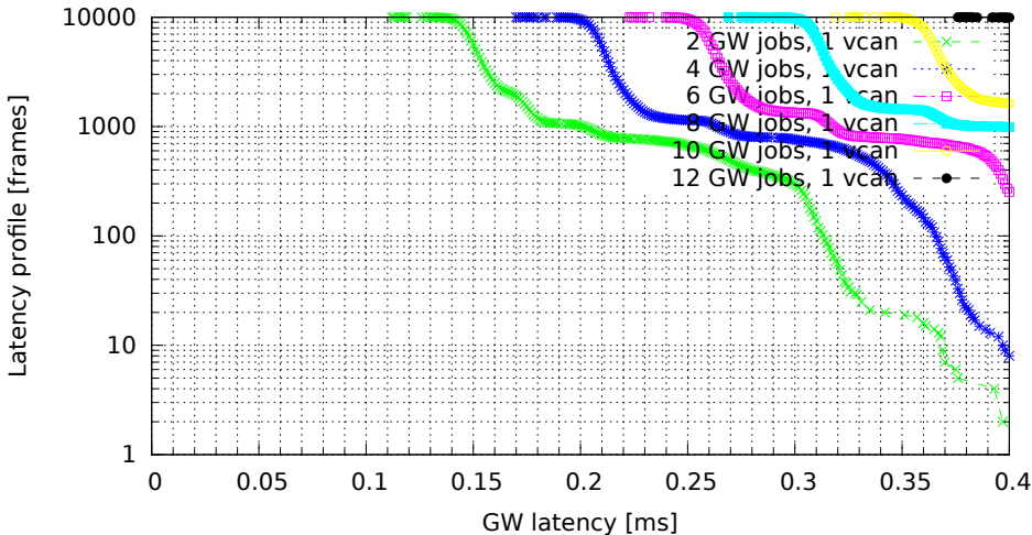
Chained GWs on a single VCAN interface (GW kernel 2.6.33.7-rt29-00004-g92487e4, Traffic onetatime, Load cpu)
