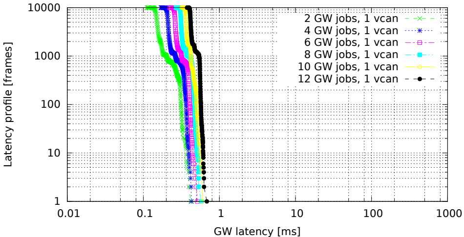
Chained GWs on a single VCAN interface (GW kernel 2.6.33.7-rt29-00004-g92487e4, Traffic oneatatime, Load cpu)
