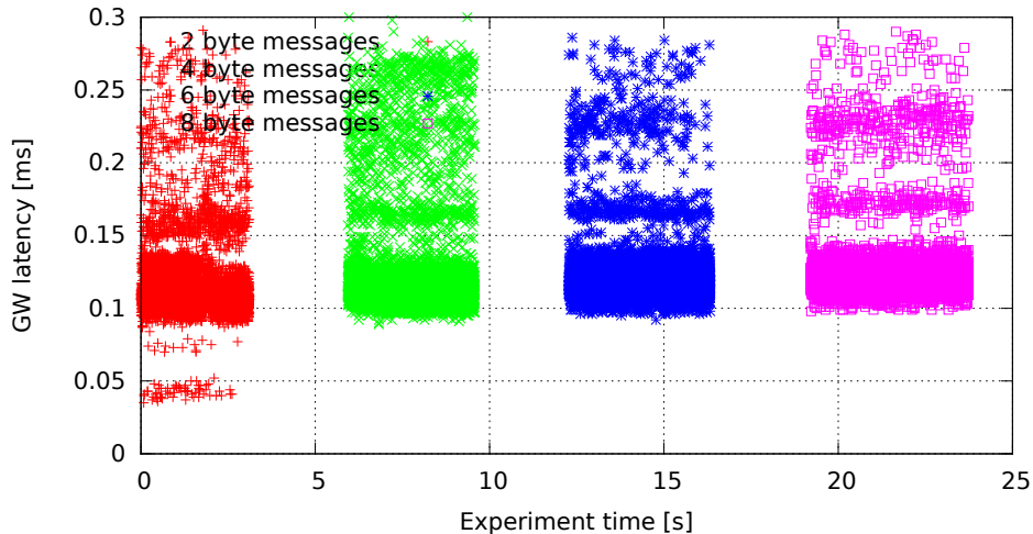
Single GW rule for all messages, no modifications (GW kernel 2.6.33.7-rt29-00004-g92487e4, Traffic oneatatime, Load cpu)
