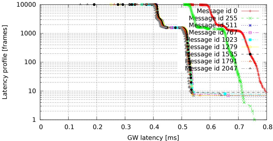
2048 GW rules (one per id, mask 0x7FF), no modifications (GW kernel 2.6.33.7-rt29-00004-g92487e4, Traffic onetatime, Load cpu)
