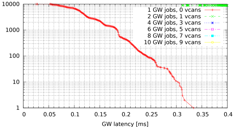
Chained GWs on multiple VCAN interfaces (GW kernel 2.6.33.7-rt29-00004-g92487e4, Traffic flood, Load none)
