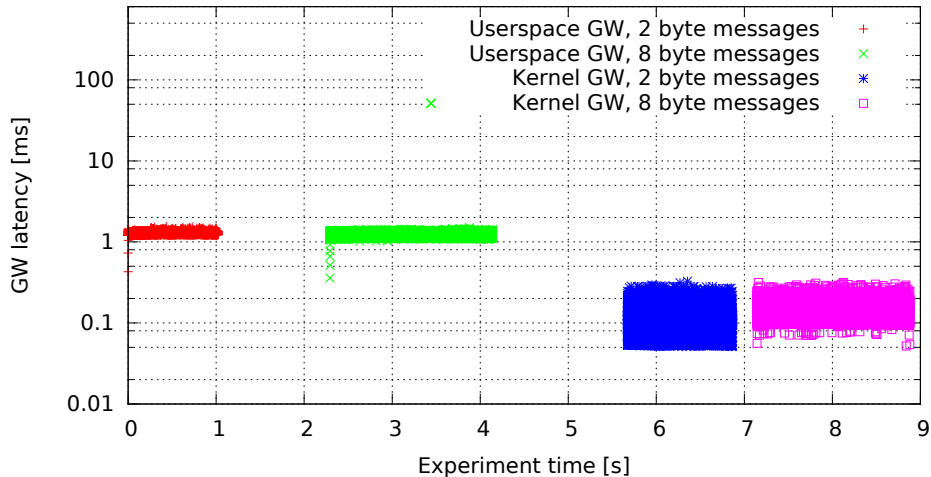
Single GW rule for all messages, no modifications (GW kernel 2.6.33.7-rt29-00004-g92487e4, Traffic flood, Load none)
