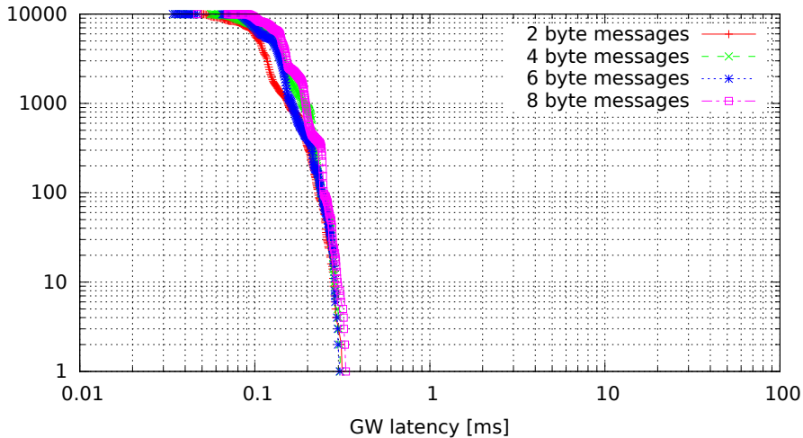
Single GW rule for all messages, no modifications (GW kernel 2.6.33.7-rt29-00004-g92487e4, Traffic flood, Load none)
