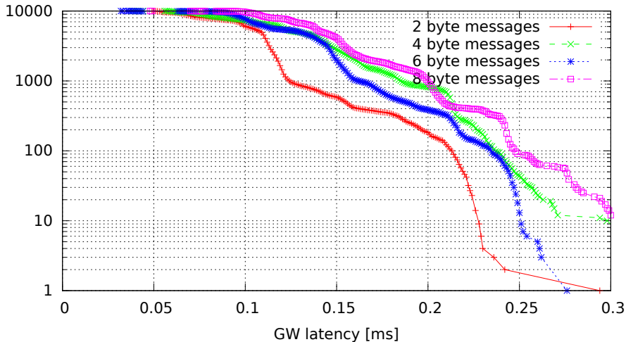
Single GW rule for all messages, no modifications, high (soft)irq task priority (GW kernel 2.6.33.7-rt29-00004-g92487e4, Traffic flood, Load none)
