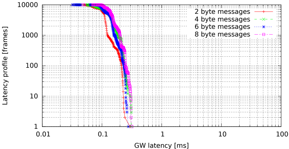
Single GW rule for all messages, no modifications, high (soft)irq task priority (GW kernel 2.6.33.7-rt29-00004-g92487e4, Traffic flood, Load none)
