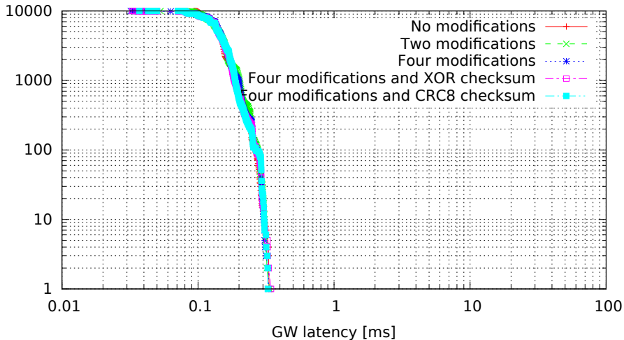
Single GW rule for all messages with modifications, 8 byte messages (GW kernel 2.6.33.7-rt29-00004-g92487e4, Traffic flood, Load none)
