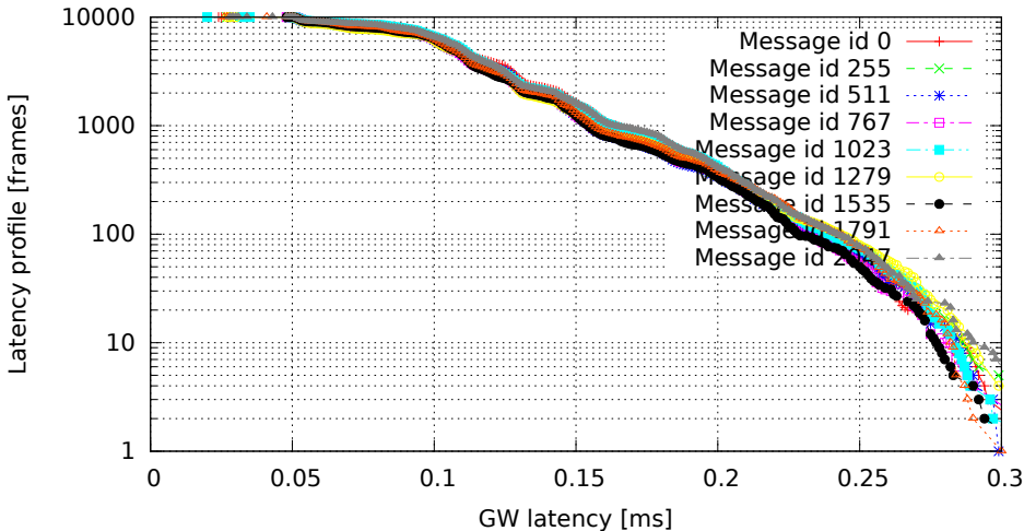
2048 GW rules (one per id, mask C00007FF), no modifications (GW kernel 2.6.33.7-rt29-00004-g92487e4, Traffic flood, Load none)
