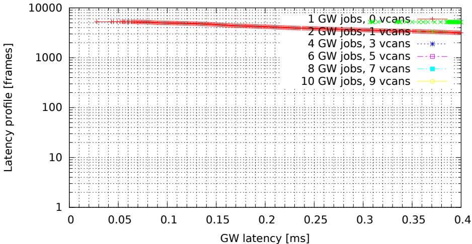
Chained GWs on multiple VCAN interfaces (GW kernel 2.6.33.7-rt29-00004-g92487e4, Traffic flood, Load eth)
