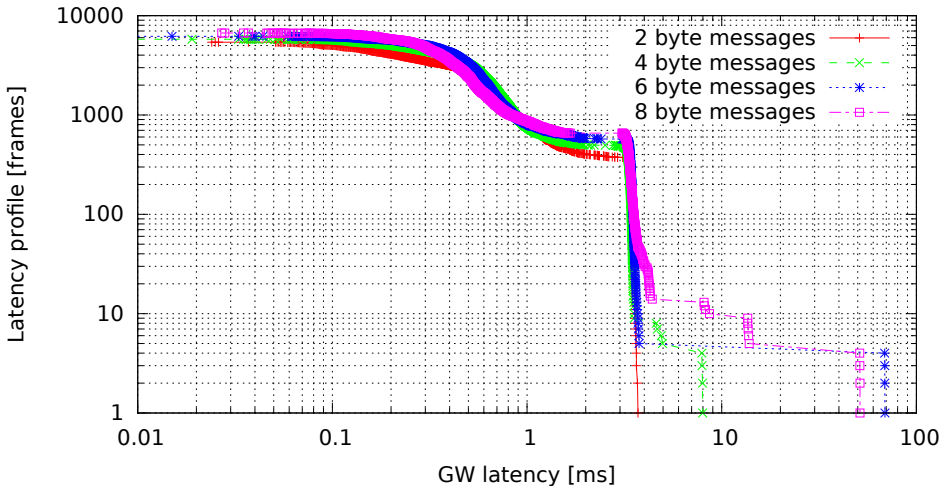
Single GW rule for all messages, no modifications (GW kernel 2.6.33.7-rt29-00004-g92487e4, Traffic flood, Load eth)
