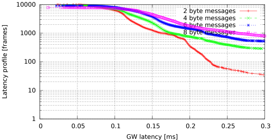
Single GW rule for all messages, no modifications, high (soft)irq task priority (GW kernel 2.6.33.7-rt29-00004-g92487e4, Traffic flood, Load eth)
