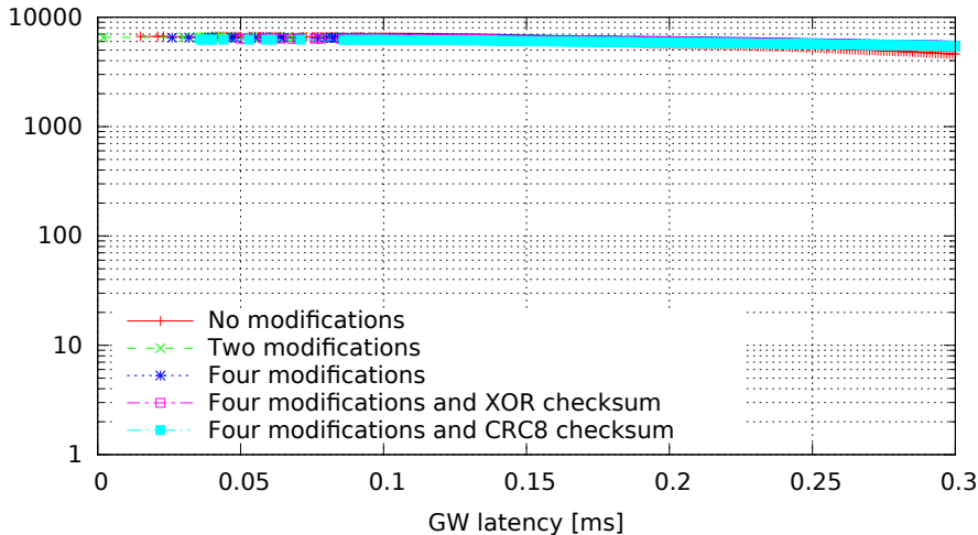
Single GW rule for all messages with modifications, 8 byte messages (GW kernel 2.6.33.7-rt29-00004-g92487e4, Traffic flood, Load eth)
