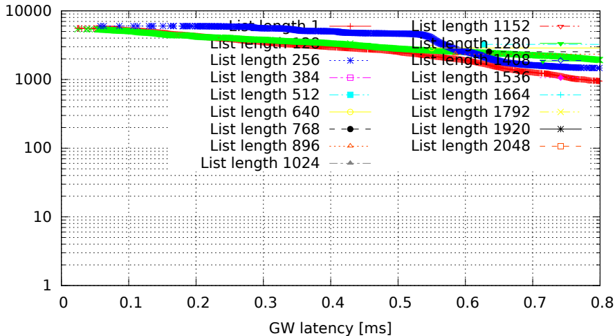
Different lengths of filter list, only the last one matches (GW kernel 2.6.33.7-rt29-00004-g92487e4, Traffic flood, Load eth)
