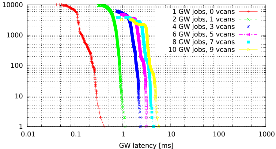
Chained GWs on multiple VCAN interfaces (GW kernel 2.6.33.7-rt29-00004-g92487e4, Traffic flood, Load cpu)
