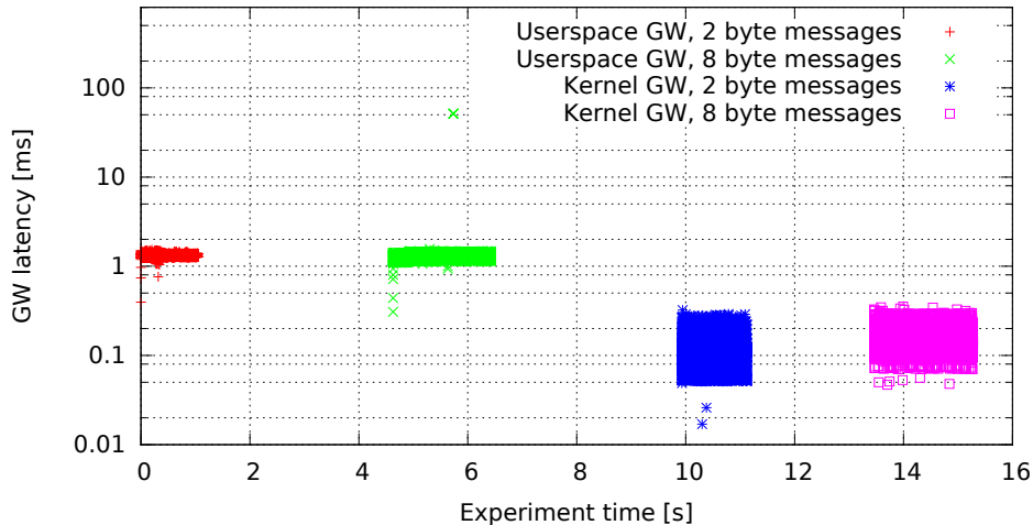
Single GW rule for all messages, no modifications (GW kernel 2.6.33.7-rt29-00004-g92487e4, Traffic flood, Load cpu)
