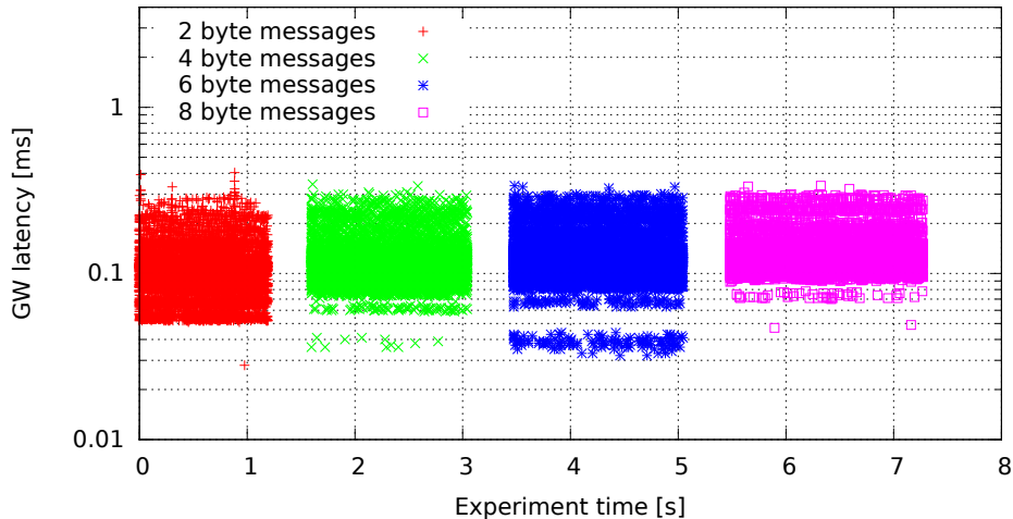
Single GW rule for all messages, no modifications (GW kernel 2.6.33.7-rt29-00004-g92487e4, Traffic flood, Load cpu)
