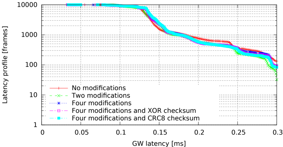
Single GW rule for all messages with modifications, 8 byte messages (GW kernel 2.6.33.7-rt29-00004-g92487e4, Traffic flood, Load cpu)
