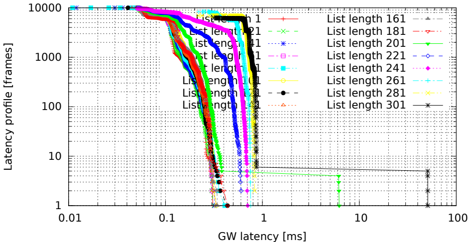
Different lengths of filter list, only the last one matches (GW kernel 2.6.33.7-rt29-00004-g92487e4, Traffic flood, Load cpu)
